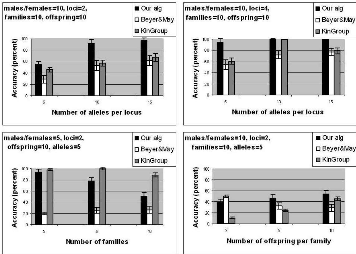
Fig. 1. Accuracy of the sibling group reconstruction using the 2-allele algorithm on randomly generated data. The y -axis shows the accuracy of reconstruction as a function of various simulation parameters. The accuracy of our algorithm is shown, as well as that of the two reference algorithms: Beyer and May, 2003 and Konovalov et al. , 2004 (KingGroup). The title shows the value of the fixed parameters: the number of adult males/females, number of families, the number of offspring per family, the number of loci, and the number of alleles per locus.
