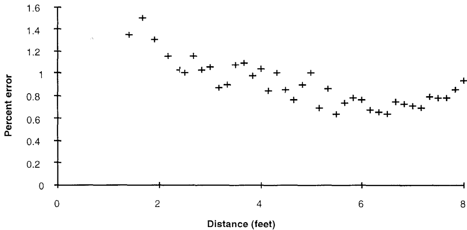
Figure 5: Percent UMD error versus distance.
