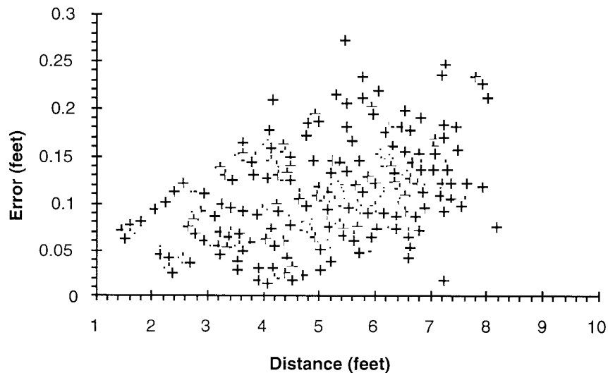
Figure 11: Errors of ERTFOB after correction
