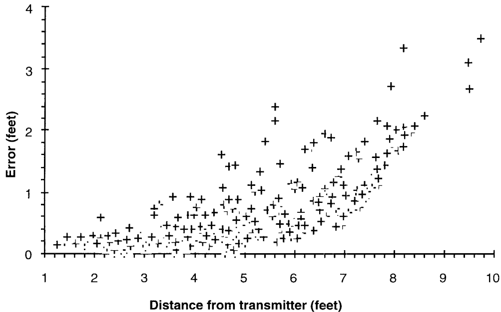
Figure 10 : ERTFOB errors measured
