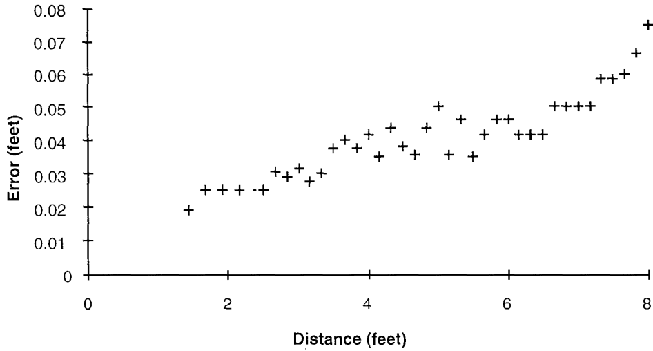
Figure 4: UMD error versus distance.
