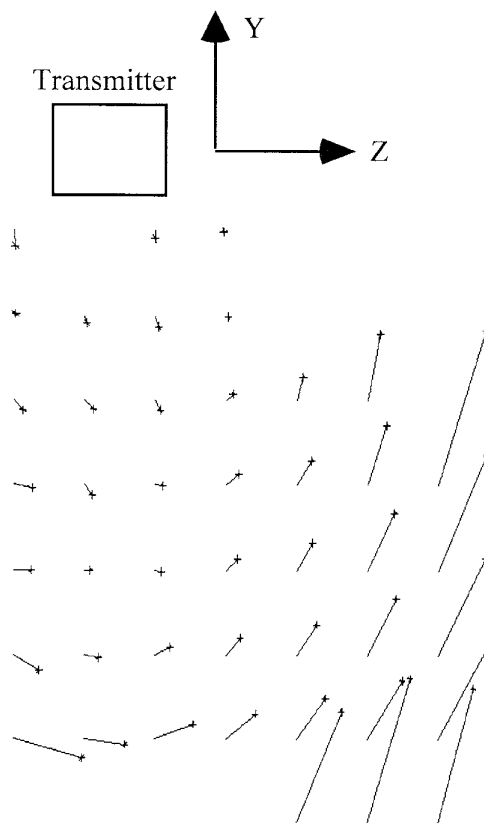
Figure 1. ERTFOB errors in one plane of the CAVE, viewed from the left side. Transmitter is one foot in front of this plane.
