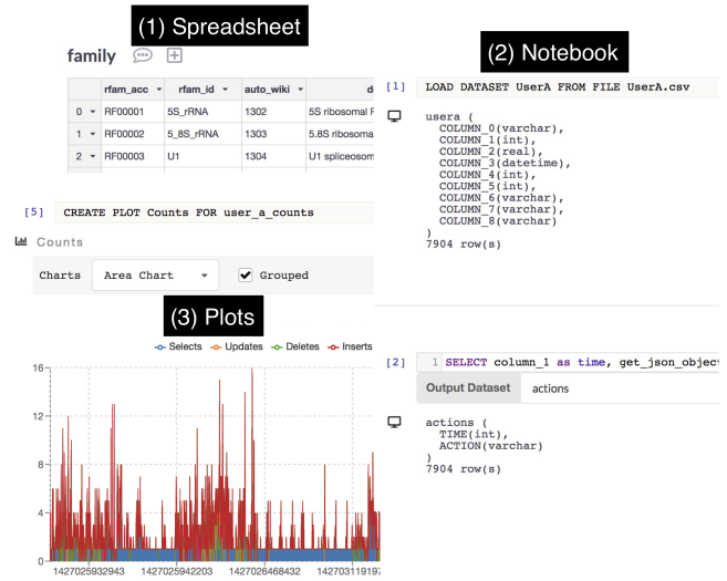
Figure 1: Vizier’s multi-modal user interface combining spreadsheets, notebooks and plots.
