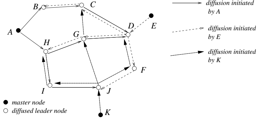
Figure 31: Illustration of time diffusion with three master nodes and n = 3 hops. The level of a node is defined with respect to each master. Outlier nodes, which do not diffuse timing messages, are not shown for simplicity. In each round, nodes take the hop-weighted (or cumulative deviation weighted) average of the different times received from the masters' diffused broadcasts.
