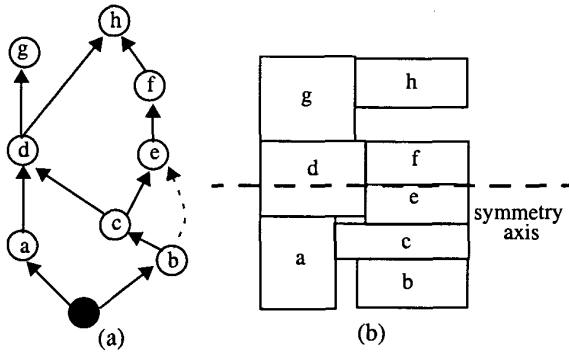
Figure 3: A symmetric y-feasible O-tree and its placement
