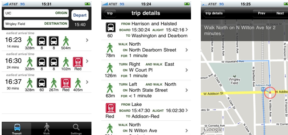
Figure 1. Screen shots from the current iPhone front-end. On the left, the main view which holds one or more route recommendations. In the middle, a route description screen. On the right, a detailed map view of a route.
