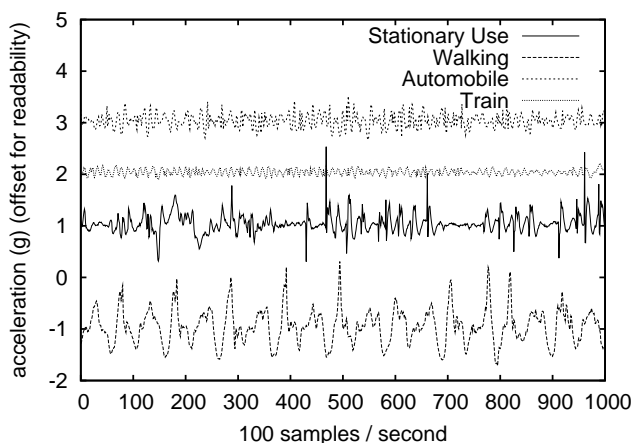
Figure 2. Accelerometer data for four types of activities.
