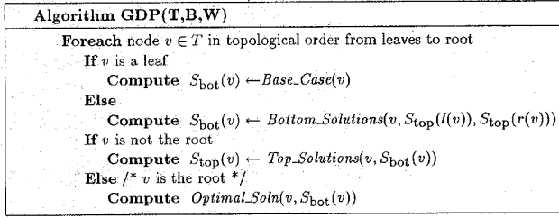
Fig. 1. General algorithm structure.
