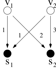
Figure 1. Sensors s_1 and s_2 will react in the same order to vertices v_1 or v_2 being contaminated. However, if v_1 is the contamination source, then the reaction delay between s_1 and s_2 is 1, while if v_2 is the source, the delay is 2.
