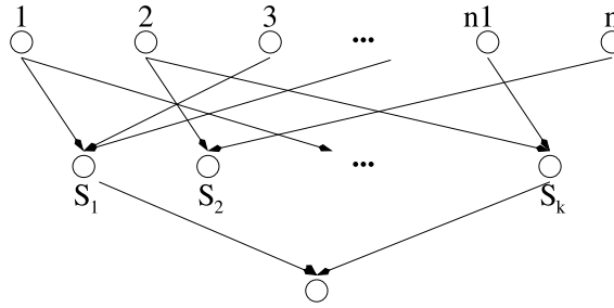
Figure 5. A graph obtained after the reduction from an instance of set cover. There is an edge from i to S_j if i \in S_j . All vertices S_j have an edge to the minimum vertex.
