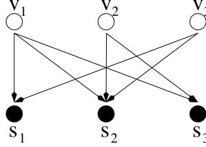
Figure 2. An example of a graph where an entire sensor sequence may be necessary for a unique contamination source identification. For each sensor s_i the incoming edges have weight i . The delay sequence for the vertices is as follows: v_1 : (s_1, 0), (s_2, 1), (s_3, 1) , v_2 : (s_2, 0), (s_3, 1) , v_3 : (s_1, 0), (s_2, 1) . For each sensor vertex s_i the delay sequence is (s_i, 0) . The minimum number of sensors for this graph is the three sensors shown in the figure.
