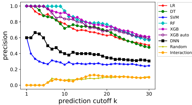
(b) Average Precision@k on test without label "doesn't matter"
