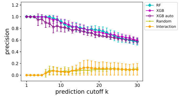
(b) Average Precision@k on test without “doesn’t matter”
