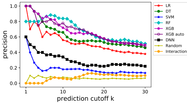
(a) Average Precision@k on full test set
