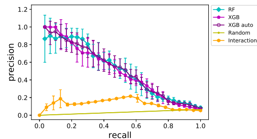
Figure 6: Precision-Recall curve for the friend-post dataset.
