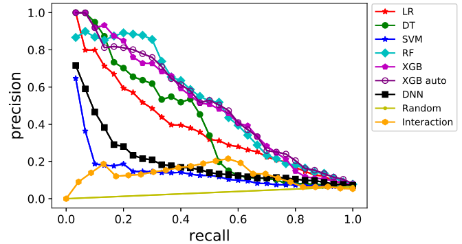
Figure 11: Precision vs. recall for the friend-post dataset.
