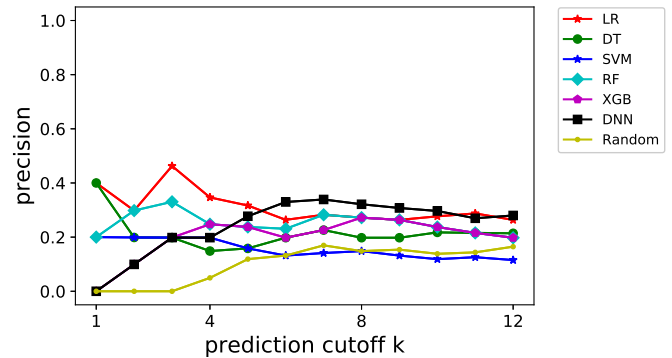
Figure 12: Average precision@k for post dataset.
