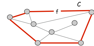
f is not in the MST
