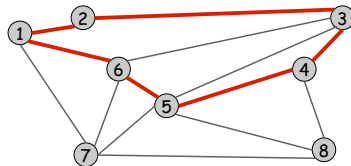
Cycle C = 1-2, 2-3, 3-4, 4-5, 5-6, 6-1
