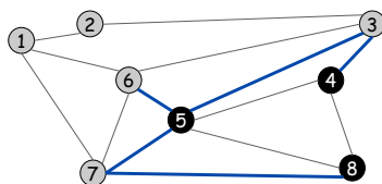
Cut S = \{4, 5, 8\} Cutset D = 5-6, 5-7, 3-4, 3-5, 7-8
