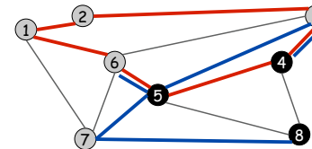
Cycle C = 1-2, 2-3, 3-4, 4-5, 5-6, 6-1 Cutset D = 3-4, 3-5, 5-6, 5-7, 7-8 Intersection = 3-4, 5-6
