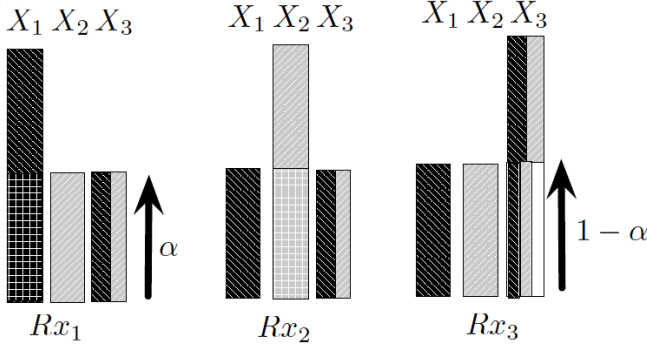
Fig. 2. LDC 3-CIFC-CMS in weak interference with \alpha = 1/2 . The achievable rates are R_1/n_d = R_2/n_d = 1, R_3/n_d = 1 - \alpha thereby achieving the sum-capacity upper bound in (8) under the condition in (10). Dark black bits are intended to Rx_1 , gray bits are intended to Rx_2 , and white bits are intended to Rx_3 .
