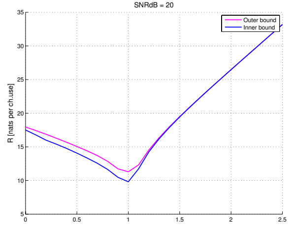
Fig. 4. Comparison of the numerically optimized inner and outer bounds for K = 3 users at \text{SNR} = 20\text{dB} as a function of \alpha = \frac{\log(|h_d|)}{\log(|h_i|)} ; notice a smaller gap than the worst case predicted 6 bits per channel use.
