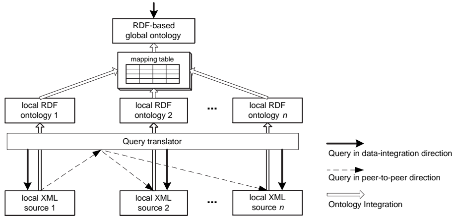
Figure 2. Architecture of the integration framework.
