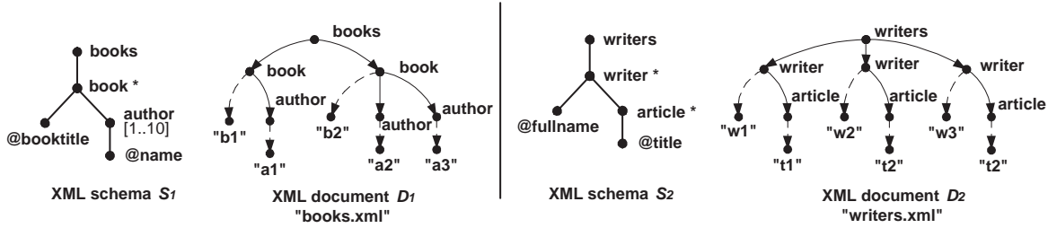
Figure 1. An example of structural heterogeneity between XML documents.
