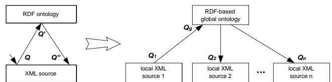
Figure 3. Query translation and reversibility.
