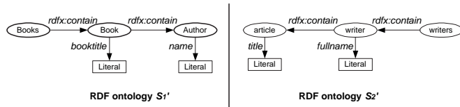
Figure 4. RDF ontologies transformed from the XML schemas in the case study.
