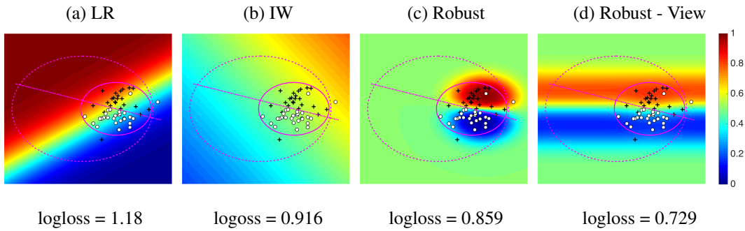
Figure 1: Comparison of Logistic Regression(a), Important Weighting Logistic Regression(b), Robust Bias-Aware Prediction(c) and View-based Robust Bias-Aware Prediction(d).
