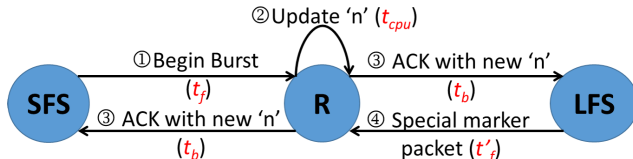
Fig. 8. DADR convergence time measurement.
