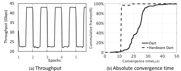
Fig. 9. Testbed measurements of DADR convergence.
