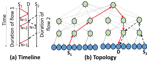
Fig. 2. Direct apportioning of sending rates.
