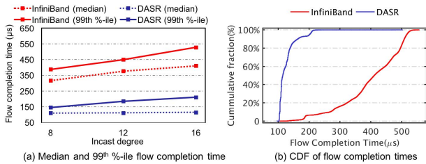
Fig. 10. Testbed flow completion latency.
