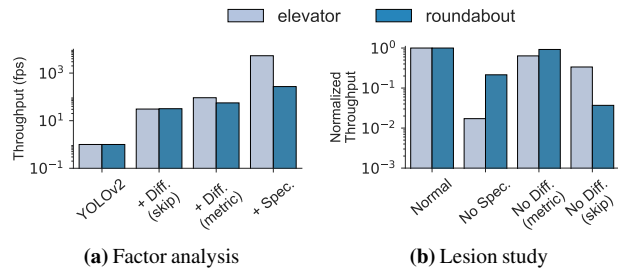
Figure 8: Factor analysis and lesion study of NOSCOPE’s filters. The factor analysis shows the impact of adding different filters for two videos; from left to right, we add each of the filters in turn over YOLOv2. The lesion study shows the impact of removing filters; the leftmost bars show normalized performance with all of NOSCOPE’s features enabled, and the remaining bars to the right show the effect of removing each filter from NOSCOPE. (Note the logarithmic scale on the y-axes of both plots.)
