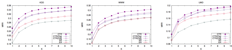
Figure: CTR that uses citation network neighbors is compared with ExpandRank (ER) that uses textually-similar neighbors and SingleRank (SR) that only uses the target document content [Wan and Xiao, 2008].
