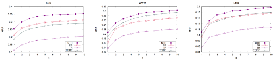
Figure: MRR curves for different keyphrase extraction methods. CTR is compared with the baselines: TFIDF, TextRank (TR) [Mihalcea and Tarau, 2004], and ExpandRank (ER) [Wan and Xiao, 2008].
