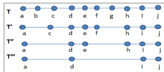
FIGURE 2- ALGORITHM TRACE
