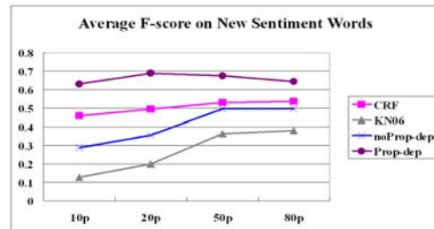
Fig. 4. F-scores of CRF , KN06 , noProp-dep and Prop-dep
