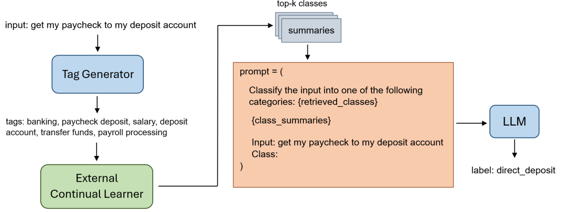
Figure 1: Overview of the InCA framework. The diagram depicts the stages of generating semantic tags for the input, identifying the most similar classes via the ECL, and constructing the prediction prompt with class summaries, which together enables efficient in-context continual learning without retaining any training data.
