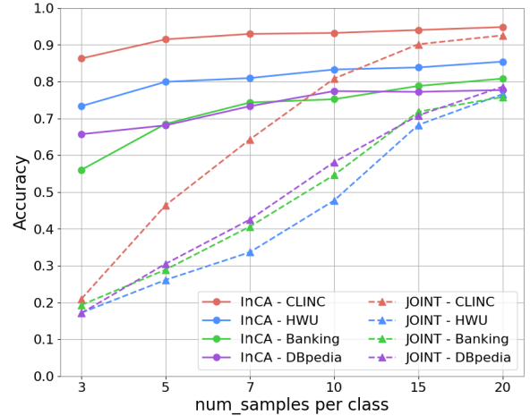
Figure 4: Performance comparison of InCA and JOINT fine-tuning across different data sizes. InCA demonstrates robust performance with limited data, particularly excelling over the fine-tuned model in data-constrained situations.
