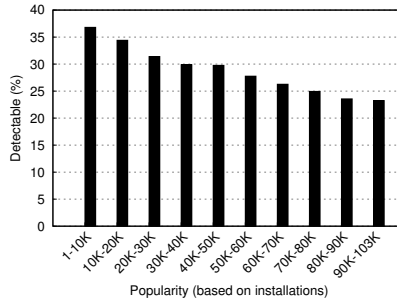
Fig. 3: Correlation of detectability of extensions and their relative popularity.
