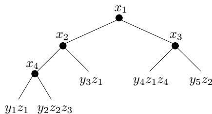
Figure 1: A non-repeating, unate-leaf decision tree (NUD)
